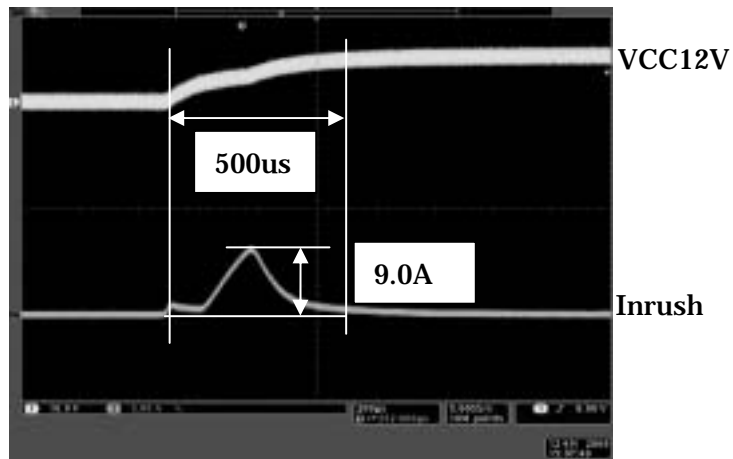
Fig.7 Inrush current
