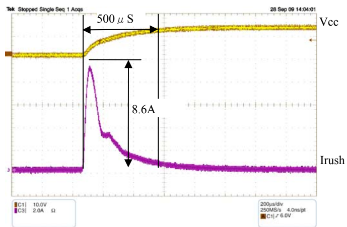
Fig.7 Inrush current
