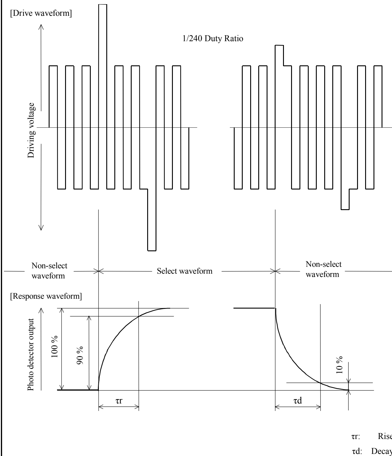
Fig.12 Definition of response time
