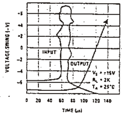
Female Follower Pulse Response
