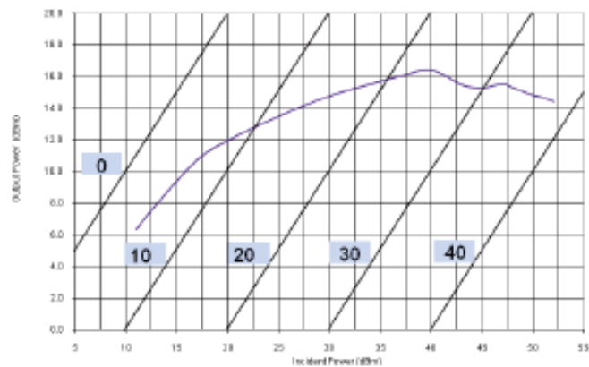
Flat Leakage Output Power vs. Input Power, Pulse width = 10 \mu s, Duty Cycle = 1%, f = 2 GHz
