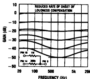
FIGURE 11. Loudness Compensated Volume Characteristic
