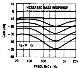
FIGURE 9. Loudness Compensated Volume Characteristic
