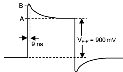
FIGURE 7. Overshoot Measurement
