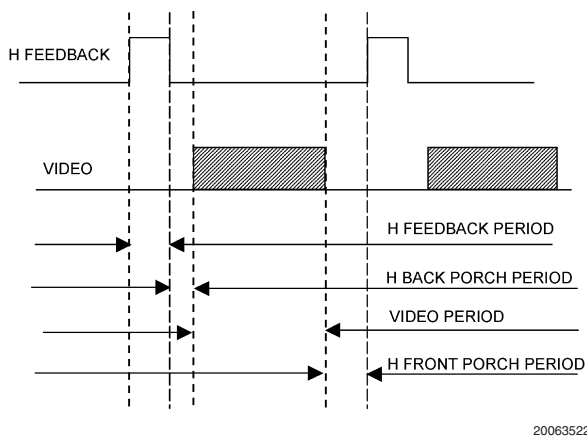
FIGURE 5. Timing Intervals with WCHE = 0
