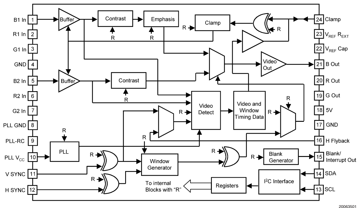
FIGURE 1. Order Number LM1270N See NS Package Number N24D
