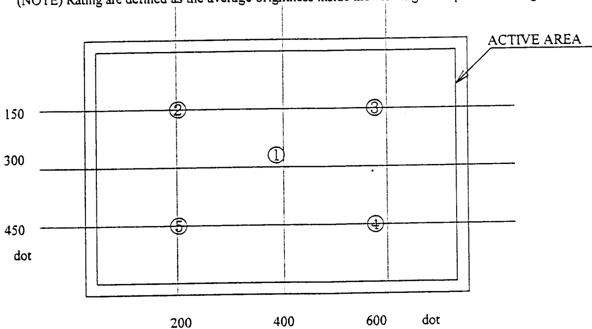
Fig.11 Measuring points (1-5)
