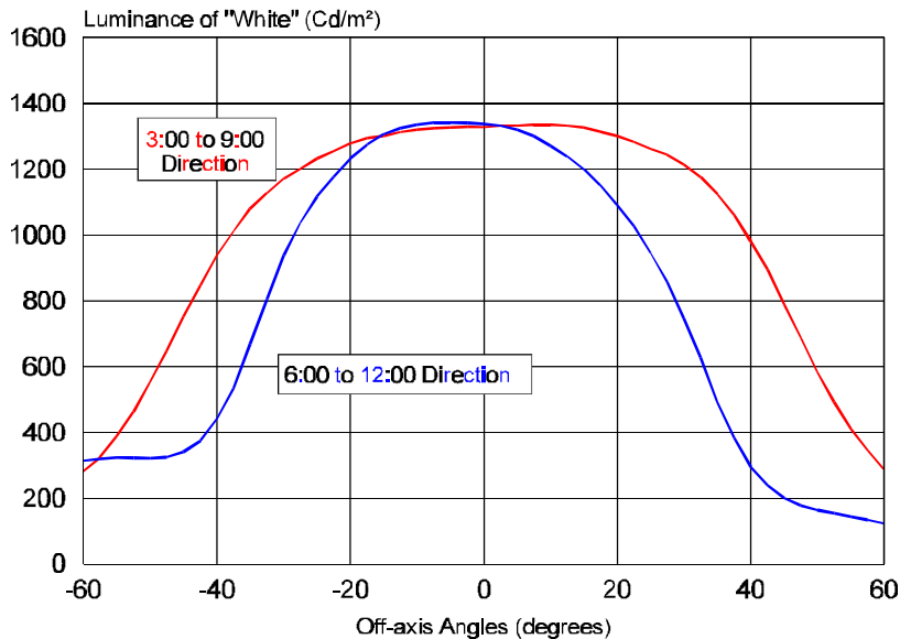
LM130A-12C318 LCD Screen Brightness Angular Distribution
