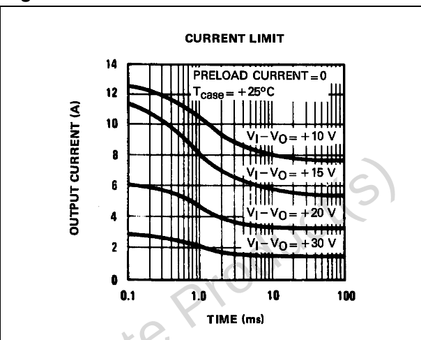
Figure 4. Current limit
