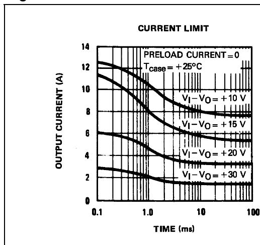
Figure 3. Current limit
