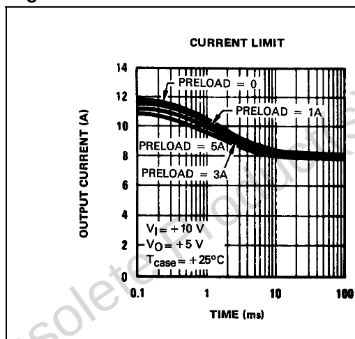
Figure 5. Current limit
