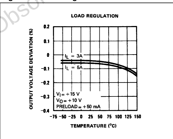
Figure 6. Load regulation
