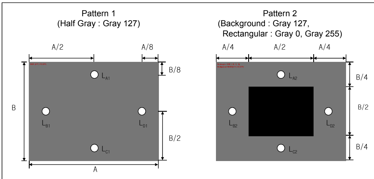
FIG. 5 Crosstalk
