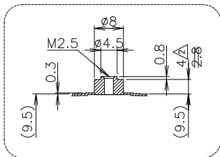
SEC D-D TWO PIECES
