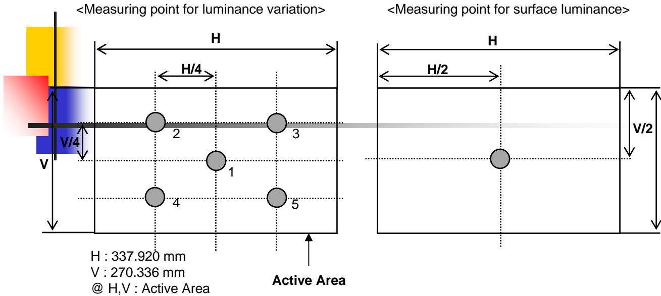
Figure 10. Luminance measuring point
