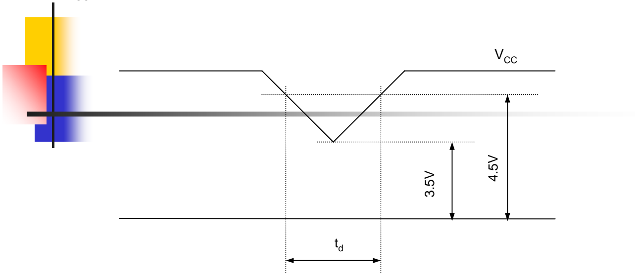
[ Figure 8 ] Power dip condition
