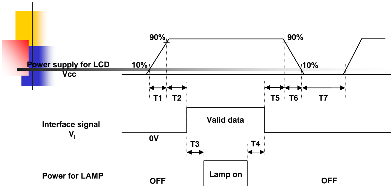
[ Figure 7 ] Power sequence
