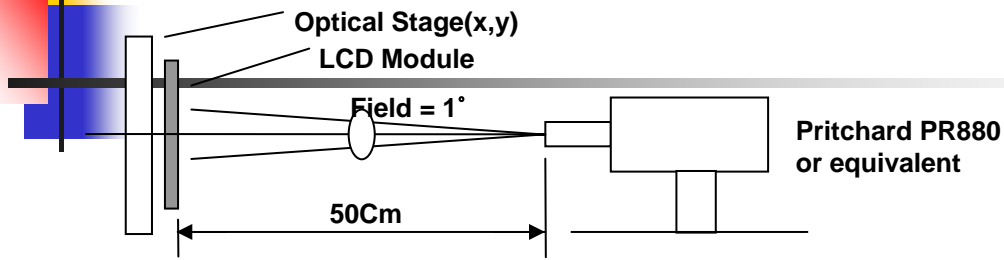
[Figure 9] Optical characteristic measurement equipment and method
