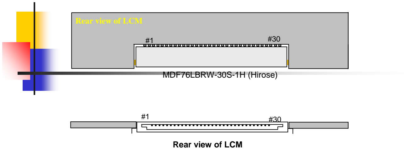
[ Figure 4 ] Connector diagram
