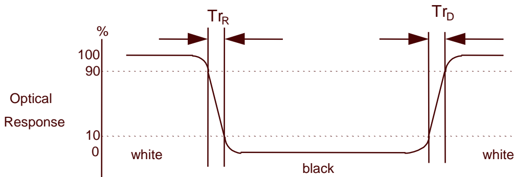
FIG. 3 Response Time
