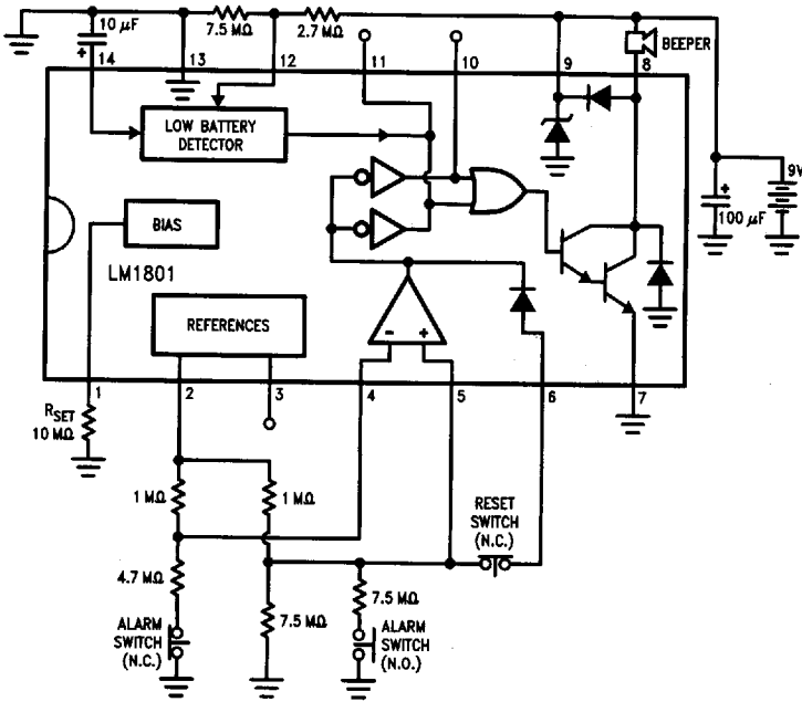
FIGURE 6. Simple Alarm Circuit
