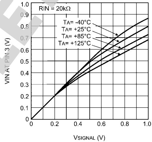
Pin 3 V_{IN} vs V_{SIGNAL} , R_{IN} = 20k\Omega
