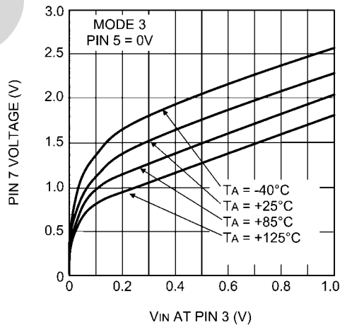
Peak Detector Voltage vs Pin 3 V IN , Mode 3
