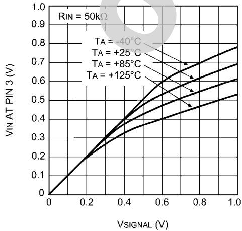
Pin 3 V_{IN} vs V_{SIGNAL} , R_{IN} = 50k\Omega
