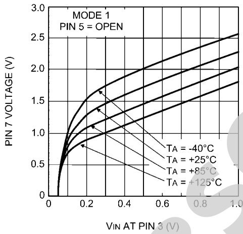
Peak Detector Voltage vs Pin 3 V IN , Mode 1
