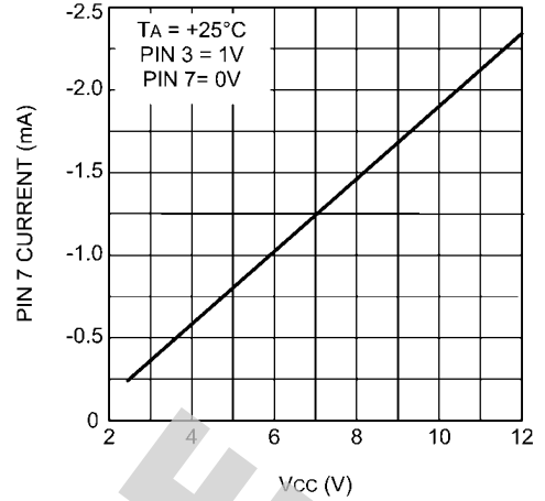
Peak Detector Charge Current vs V CC
