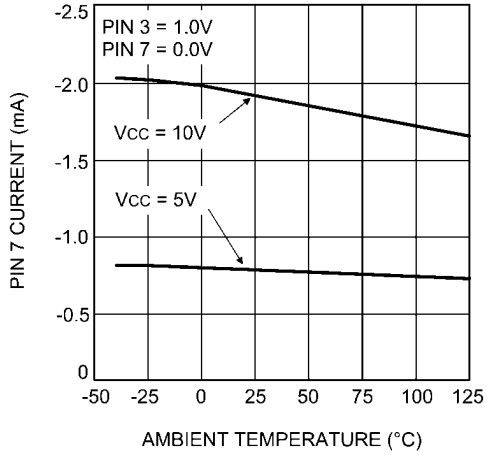
Peak Detector Charge Current vs Temperature
