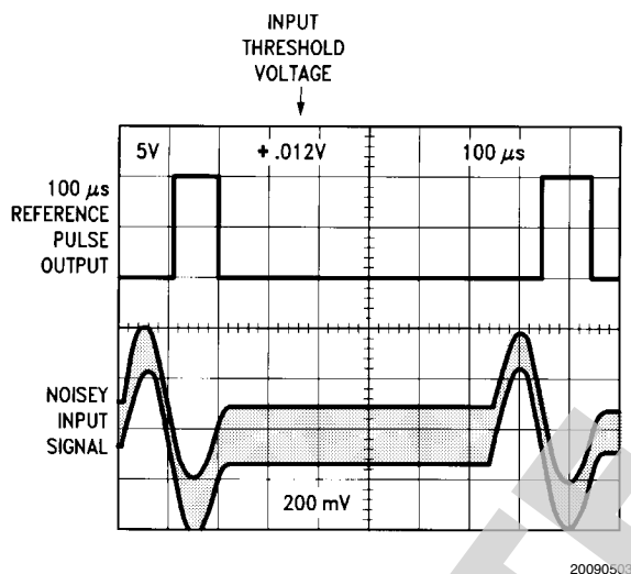
FIGURE 2. LM1815EP Oscillograms
