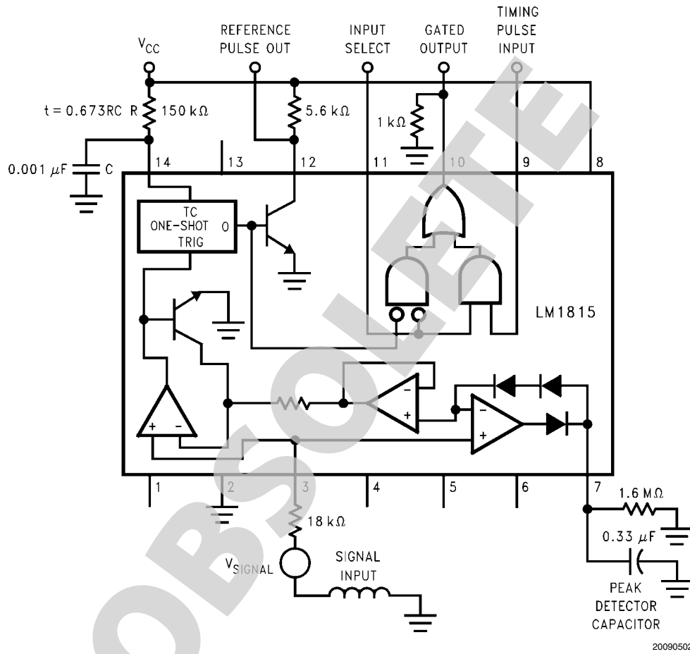
FIGURE 1. LM1815EP Adaptive Sense Amplifier
