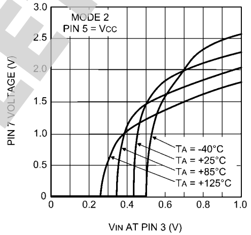
Peak Detector Voltage vs Pin 3 V IN , Mode 2
