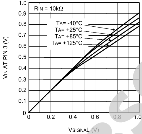
Pin 3 V_{IN} vs V_{SIGNAL} , R_{IN} = 10k\Omega
