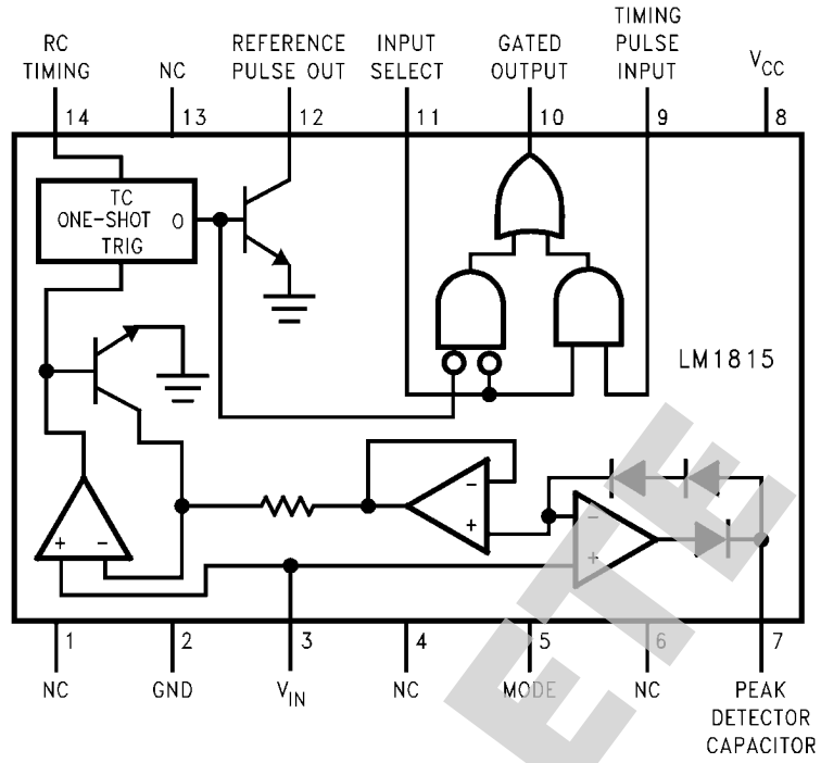
Top View See NS Package Number M14A or N14A
