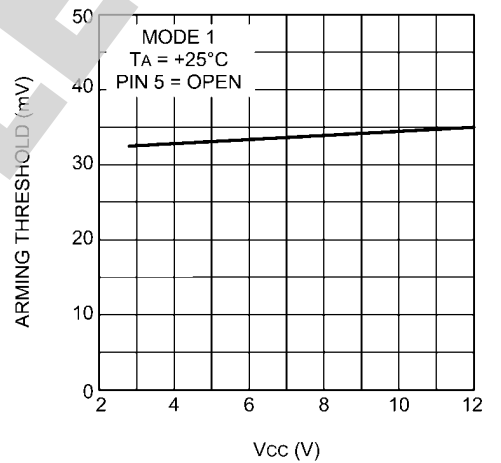
Mode 1 Minimum Arming Threshold vs V CC
