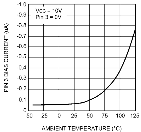
Pin 3 Bias Current vs Temperature
