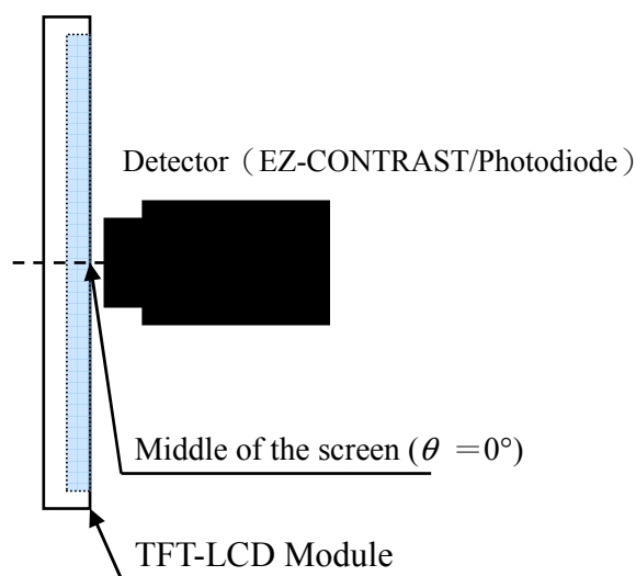
Measurement of viewing angle range, Response time.
