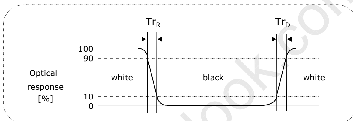
FIG. 9 Response time
