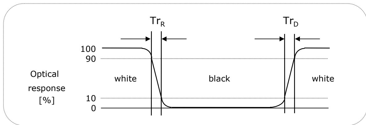
FIG. 9 Response time
