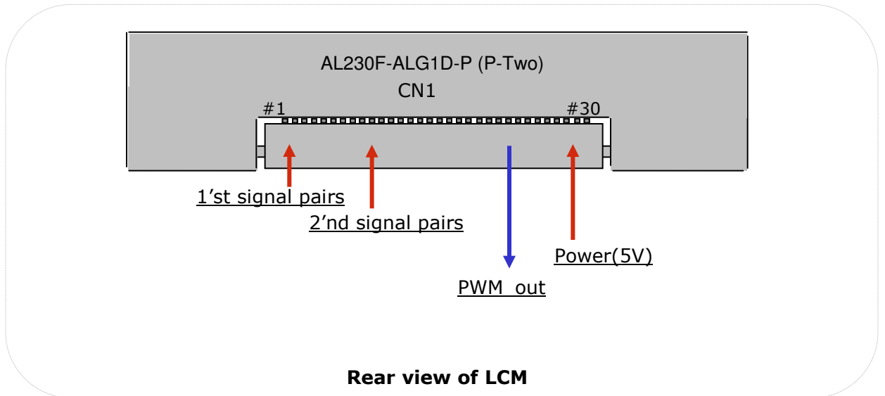
FIG. 4 Connector diagram
