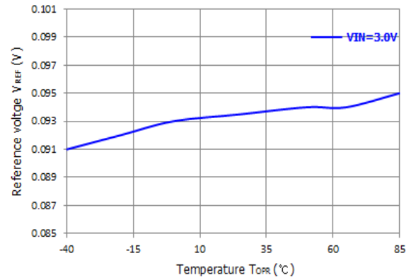
Reference voltage vs Temperature (VOUT=15V)
