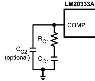
FIGURE 4. Compensation Network for LM20333A
