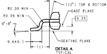
20-Lead eTSSOP Package NS Package Number MXA20A
