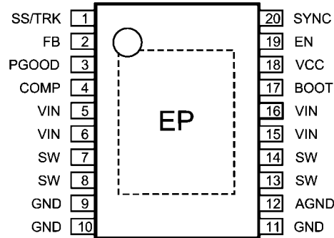
Top View eTSSOP-20 Package
