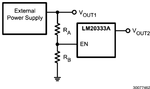
FIGURE 5. Sequencing LM20333A with Precision Enable
