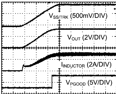
TIME (10 ms/DIV)
