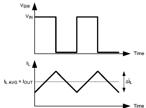
FIGURE 2. Switch and Inductor Current Waveforms
