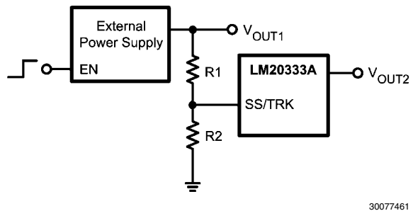
FIGURE 6. Tracking an External Supply
