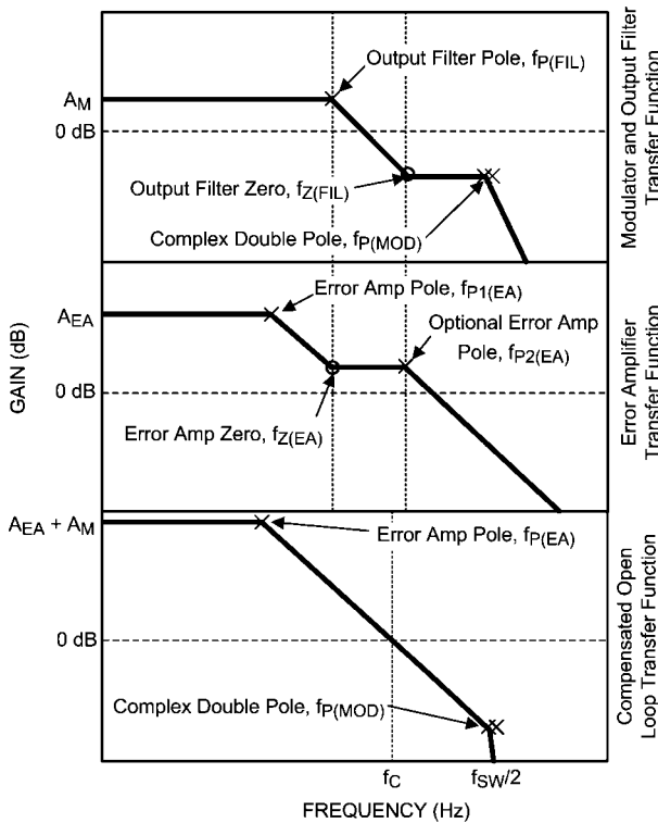
FIGURE 3. LM20333A Loop Compensation
