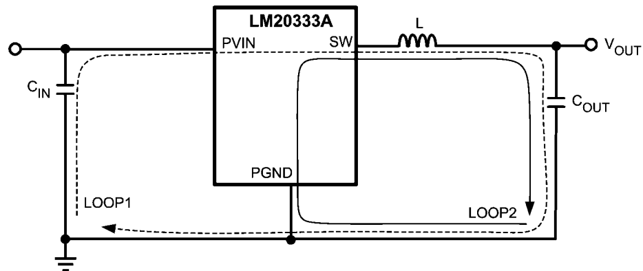
FIGURE 13. Schematic of LM20333A Highlighting Layout Sensitive Nodes
