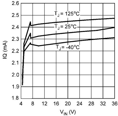
www.DataSheet4U.com Non-Switching I_Q vs. V_{IN}
