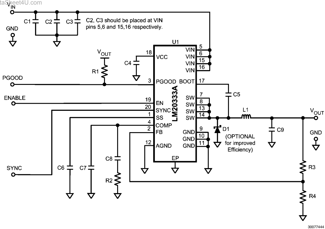
FIGURE 14. Typical Application Schematic
