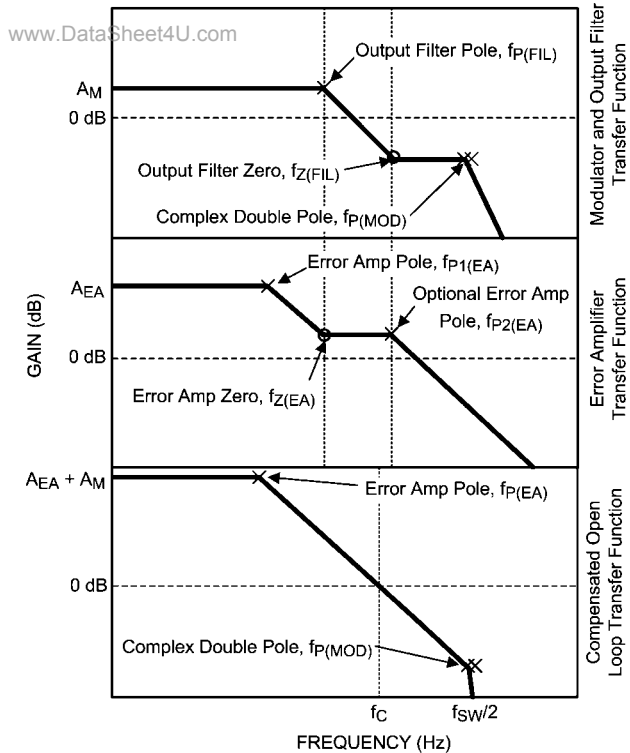
FIGURE 3. LM20333 Loop Compensation
