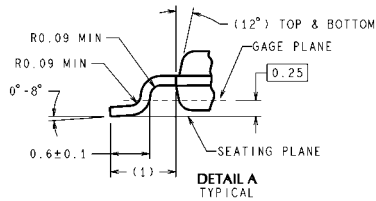
20-Lead eTSSOP Package NS Package Number MXA20A
