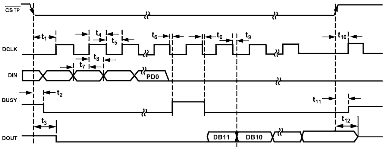
Timing diagram
