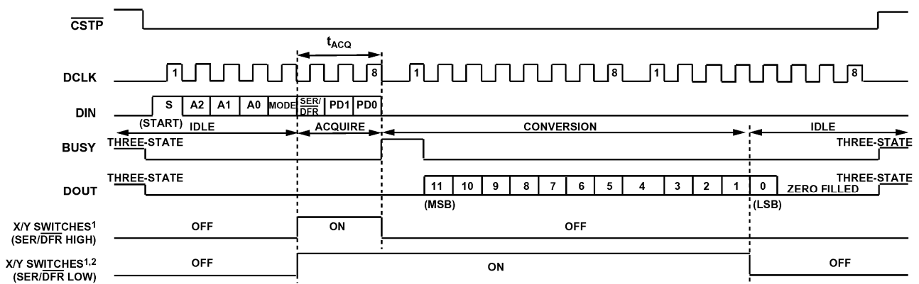
Serial Data Sequence
