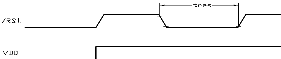
Reset Timing Diagram
