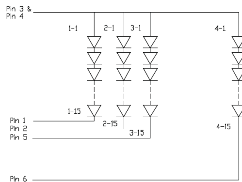
Electrical Circuit of lightbar
