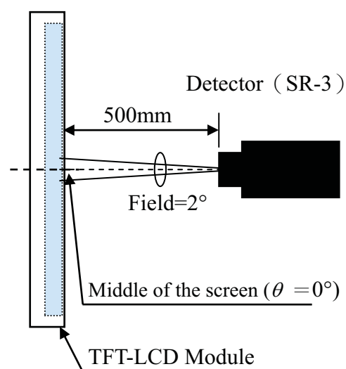
Measurement of Contrast, Luminance, Chromaticity.
