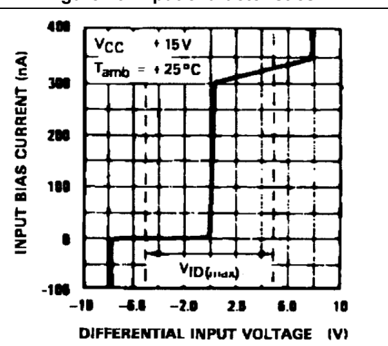
Figure 13. Input characteristics
