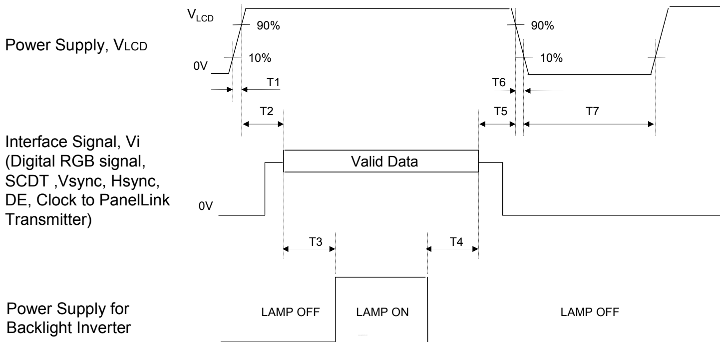
[ Figure 6 ] Power sequence
