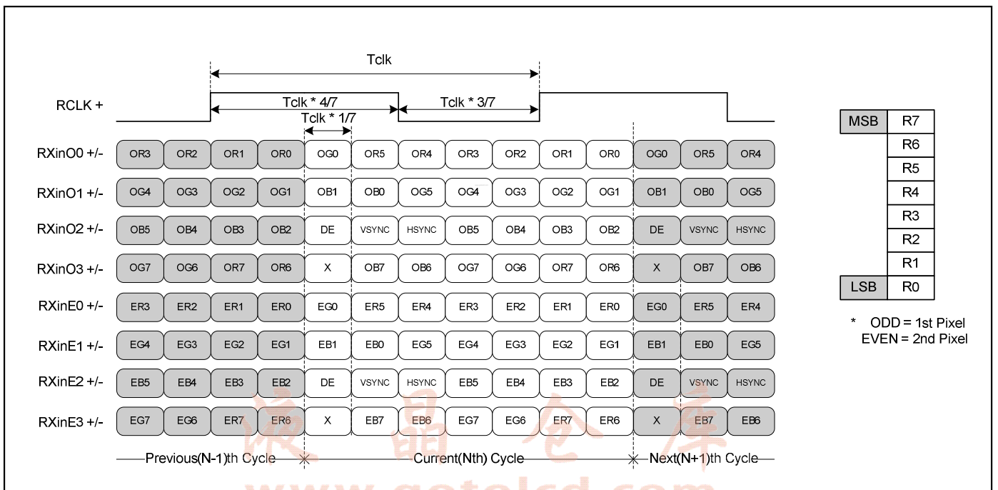
< LVDS Data Format >
