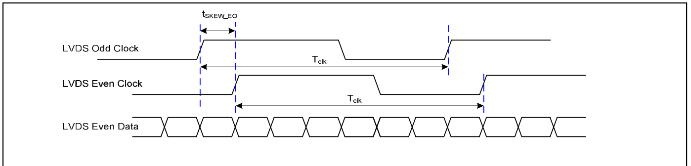
< Clock skew margin between channel >
