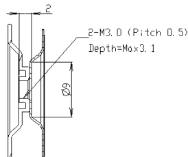
SECTION B-B SCALE 2/1
