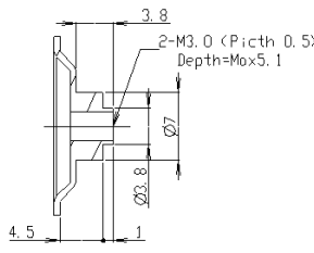
SECTION B-B SCALE 2/1
