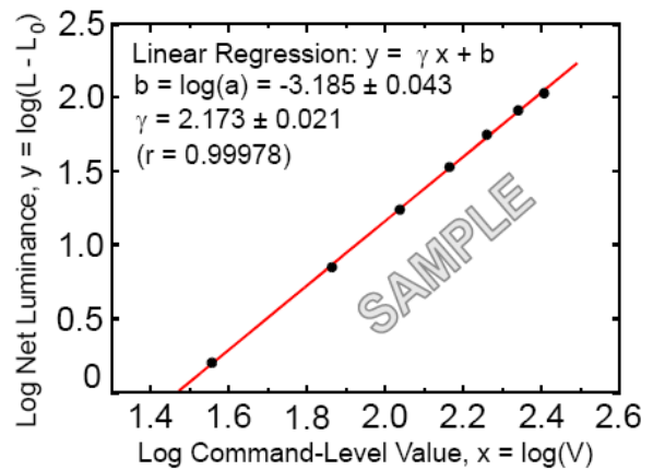
FIG. 6 Sample Log-log plot of luminance vs. gray scale
