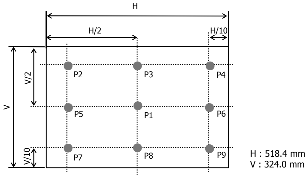
FIG. 2 Measure Point for Luminance
