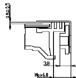
SECTION B-B SCALE 2/1
