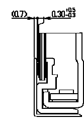
SECTION D-D SCALE 2/1
