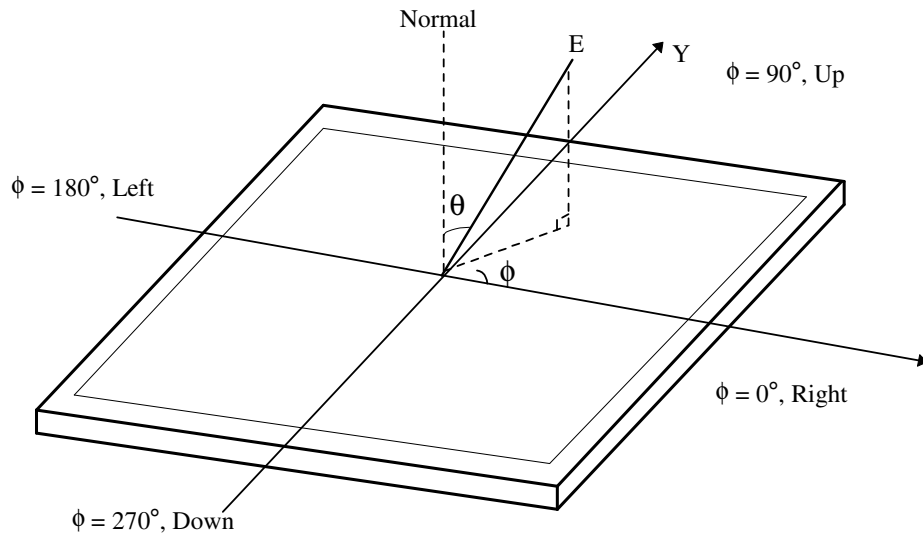
FIG. 4 Viewing angle
