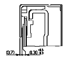
SECTION C-C SCALE 2/1
