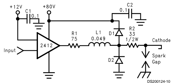
FIGURE 9. One Channel of the LM2412A with the Recommended Arc Protection Circuit.
