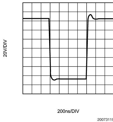
FIGURE 12. Cathode Pulse Response
