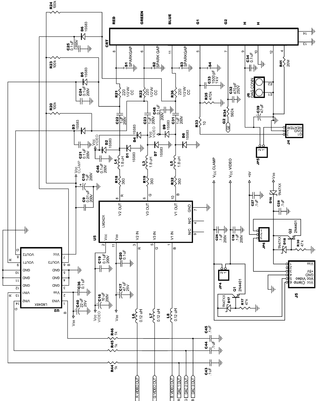
FIGURE 15. LM262X/LM242X/LM248X Demonstration Board Schematic (continued)
