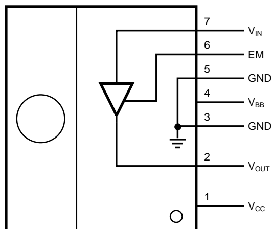
Figure 1. Simplified Connection and Pinout Diagram (Top View)
