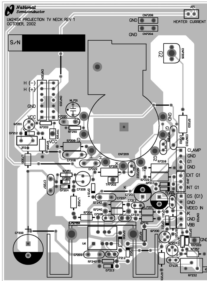
Figure 15. LM2459 Demonstration Board Layout
