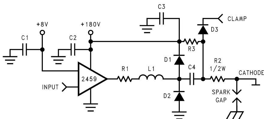
Figure 13. Recommended Application Circuit
