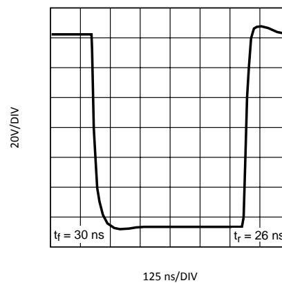
Figure 5. LM2459 Pulse Response
