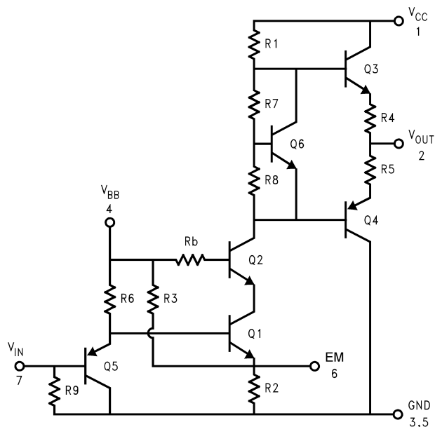
Figure 2. Simplified Schematic Diagram
