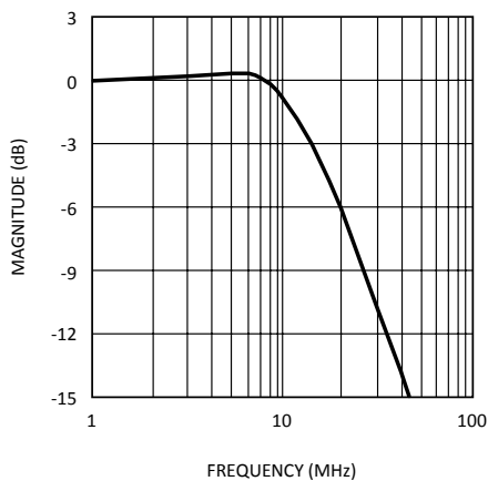
Figure 6. Bandwidth
