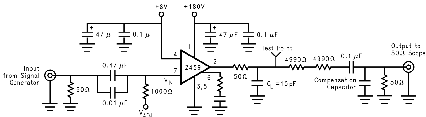
Figure 3. Test Circuit
