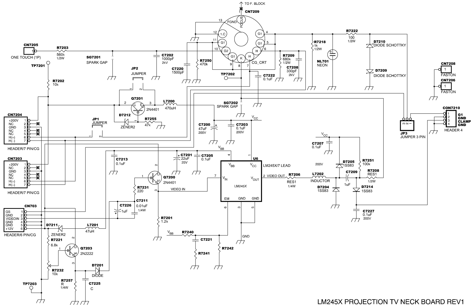
Figure 14. LM2459 Demonstration Board Schematic
