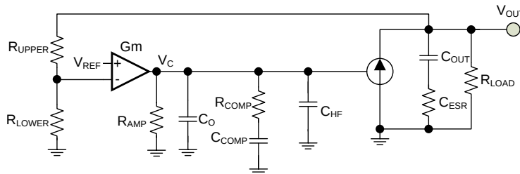
Figure 35. Transconductance Amplifier
