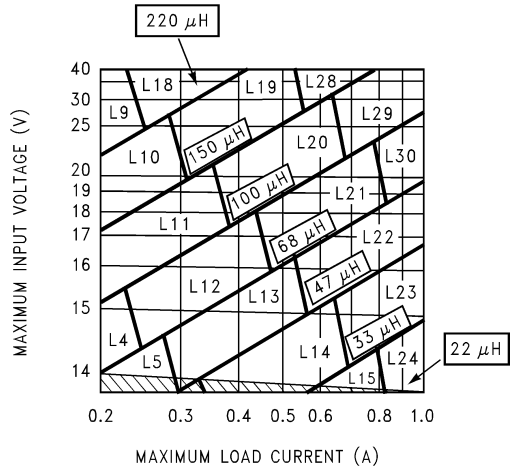
FIGURE 6. LM2675-12EP
