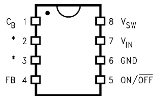
SO-8/DIP Package See NSC Package Drawing Number MO8A/N08E
