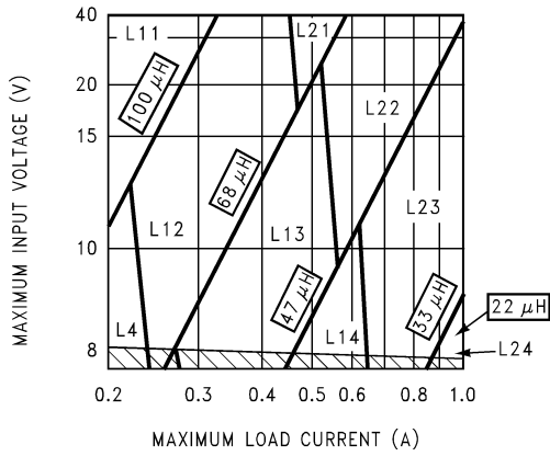
FIGURE 4. LM2675-3.3EP
