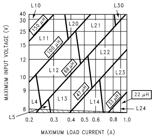
FIGURE 5. LM2675-5.0EP
