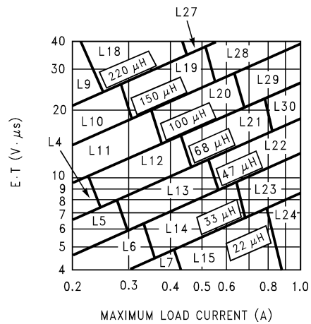
FIGURE 7. LM2675-ADJEP
