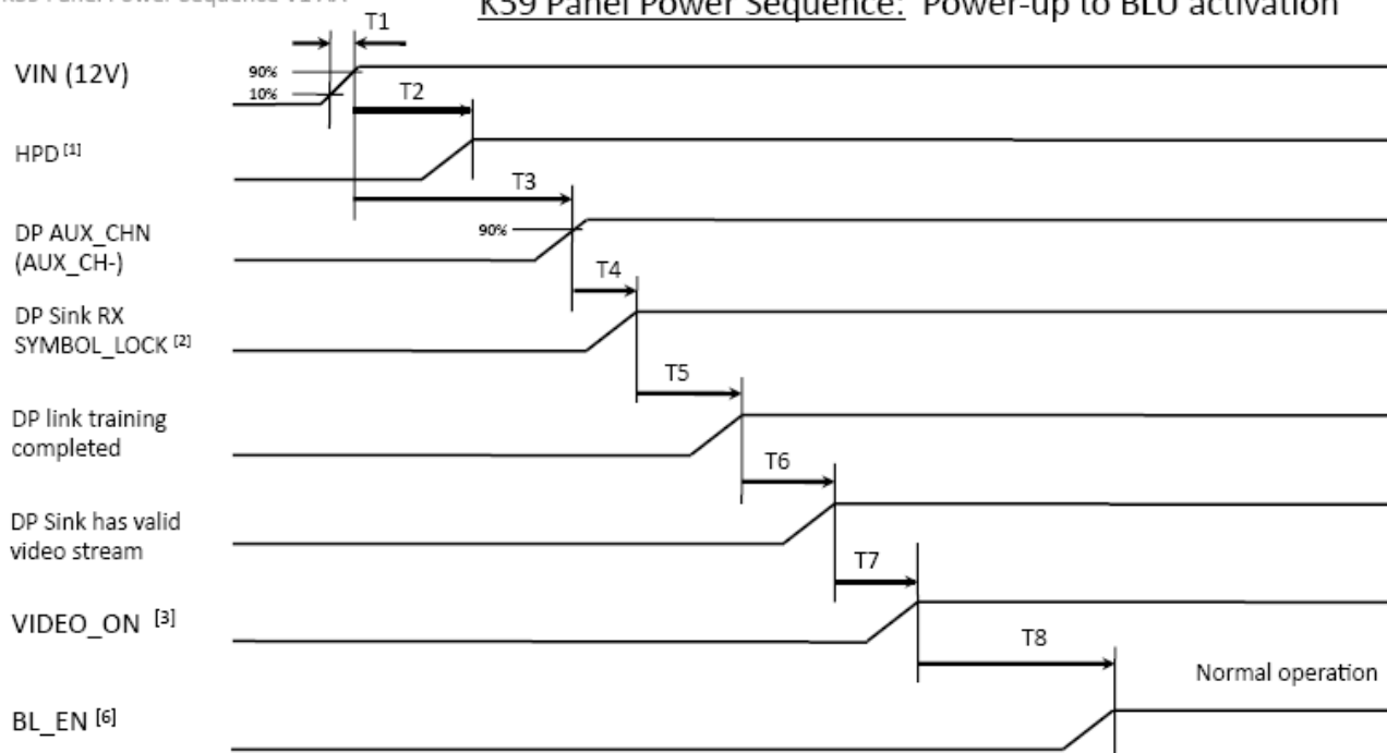
K59 Panel Power Sequence V1 AA
