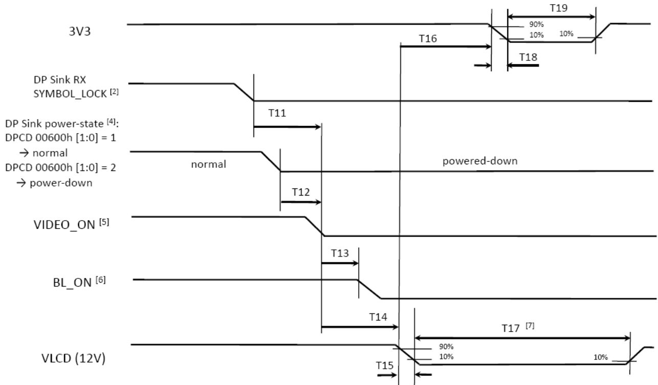
Panel Power Sequence: BL_ON de-activation
