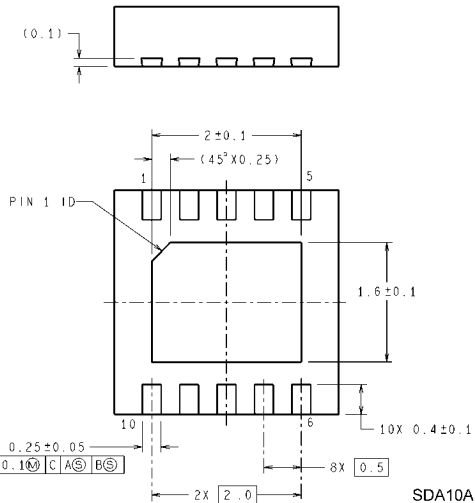
SDA10A: 10-Pin Non-Pullback Leadless Leadframe Package 3.0mm × 3.0mm × 0.8mm
