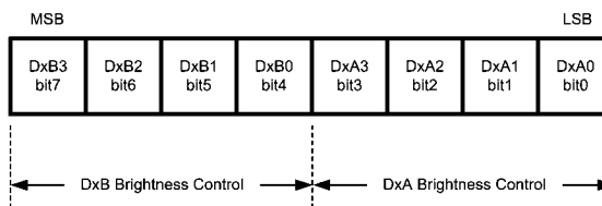
FIGURE 7. Brightness Control Register Description Internal Hex Address: A0h
