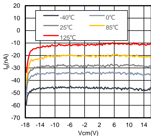
Figure 1. I_B vs. V_{CM} , ( V_+ = 18\text{ V} , V_- = -18\text{ V} )
