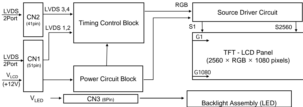
FIG. 1 Block diagram
