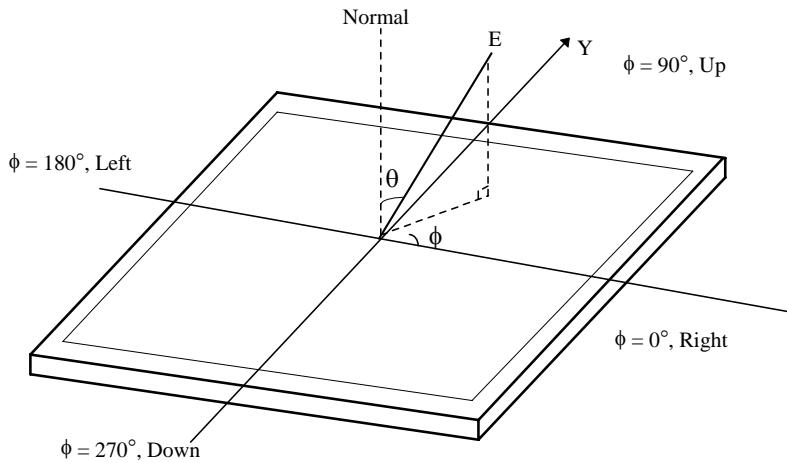
Figure 10. Viewing Angle
