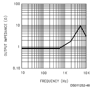
Output Impedance ( V_{stby} )
