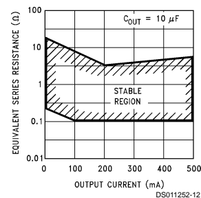
Output Capacitor ESR (Main Output, Pin 11)
