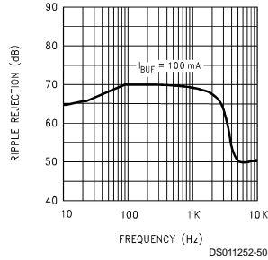
Ripple Rejection ( V_{BUF} )
