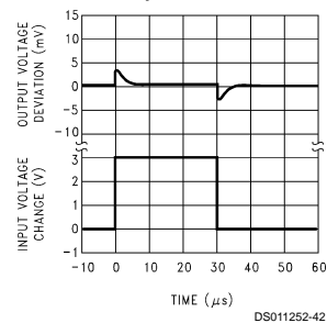
Line Transient Response ( V_{stby} )
