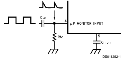
FIGURE 2. Monitoring Square Wave \mu\text{P} Signals
