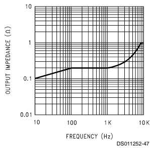
Output Impedance ( V_{buf} )
