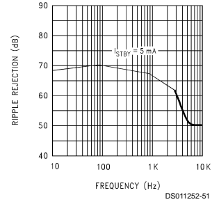
Ripple Rejection ( V_{STBY} )
