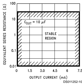
Output Capacitor ESR (Standby Output, Pin 9)
