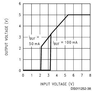
Low Voltage Behavior ( V_{buf} )
