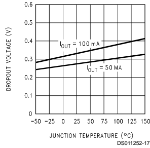
Dropout Voltage ( V_{buf} )
