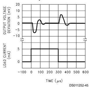
Load Transient Response ( V_{stby} )
