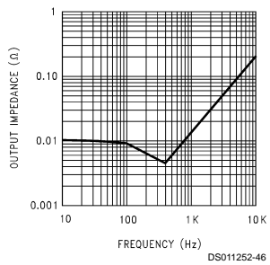
Output Impedance ( V_{OUT} )
