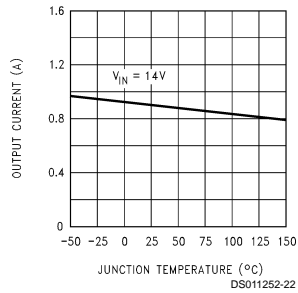
Peak Output Current ( V_{OUT} )
