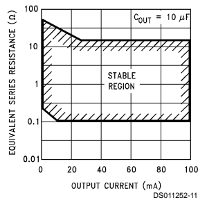
Output Capacitor ESR (Buffer Output, Pin 10)
