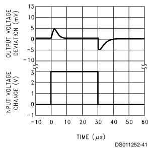
Line Transient Response ( V_{buf} )
