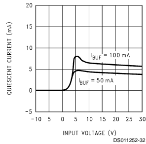
Quiescent Current ( V_{buf} )
