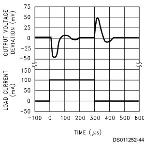
Load Transient Response ( V_{buf} )
