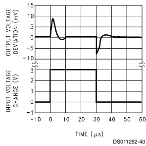
Line Transient Response ( V_{OUT} )
