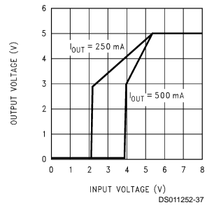
Low Voltage Behavior ( V_{OUT} )
