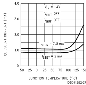
Quiescent Current ( V_{stby} )
