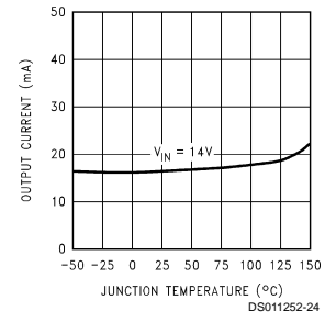
Peak Output Current ( V_{stby} )
