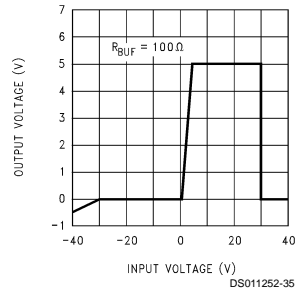
Output Voltage ( V_{buf} )
