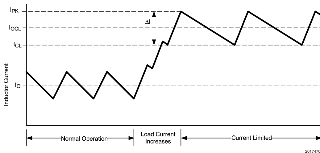
FIGURE 2. Inductor Current - Current Limit Operation
