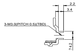
SECTION D-D SCALE 2/1
