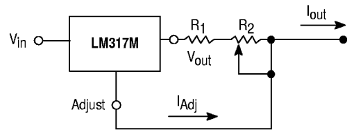
Figure 22. Current Regulator
