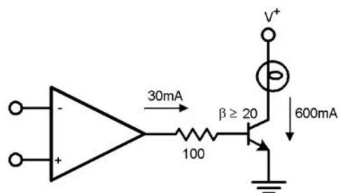
Lamp Driver
