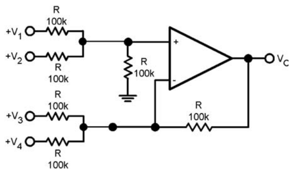
DC Summing Amplifier (V IN 's ≥ 0 V DC and V O ≥ V DC )
