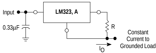
Figure 13. Current Regulator
