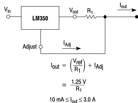
Figure 25. Current Regulator
