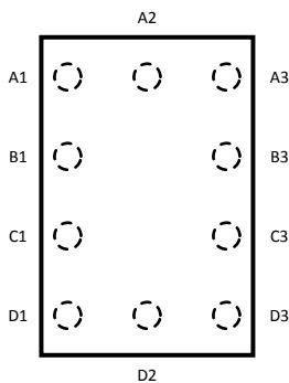
Figure 2. TOP VIEW
