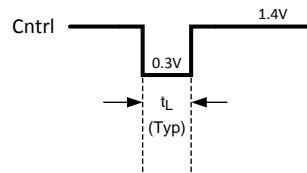
Figure 6. Control Signal Waveform
