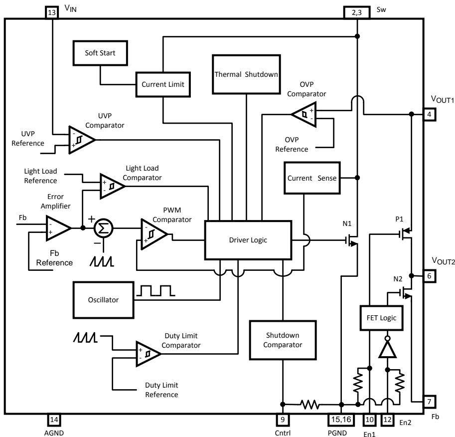
Figure 4. Block Diagram
