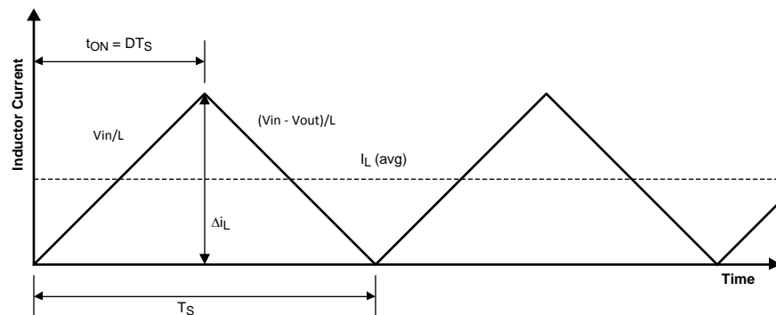
Figure 7. Inductor Current Waveform
