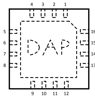
Figure 3. TOP VIEW
