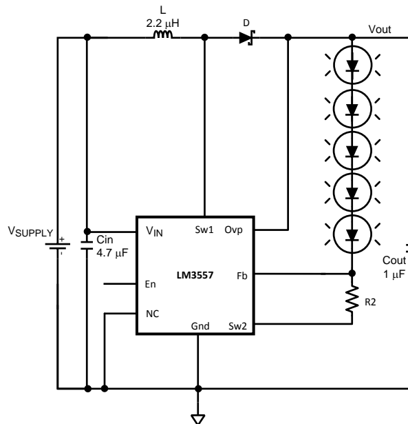
Figure 1. Backlight Configuration
