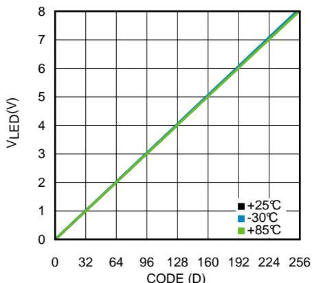
Figure 21. ADC Linearity
